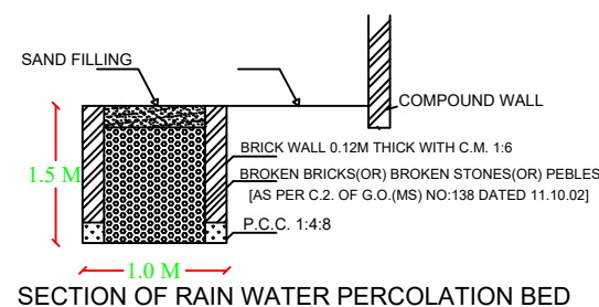
SECTION OF RAIN WATER PERCOLATION BED
