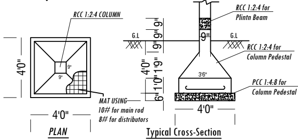
FOOTING DETAILS
