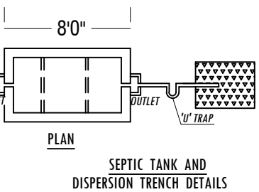
SEPTIC TANK AND DISPERSION TRENCH DETAILS
