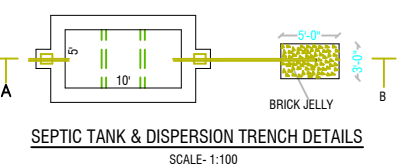
SEPTIC TANK & DISPERSION TRENCH DETAILS SCALE- 1:100
