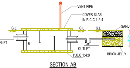
SECTION-AB
