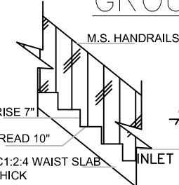
STAIRCASE DETAILS SCALE- 1:20
