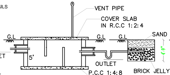
SECTION-AB
