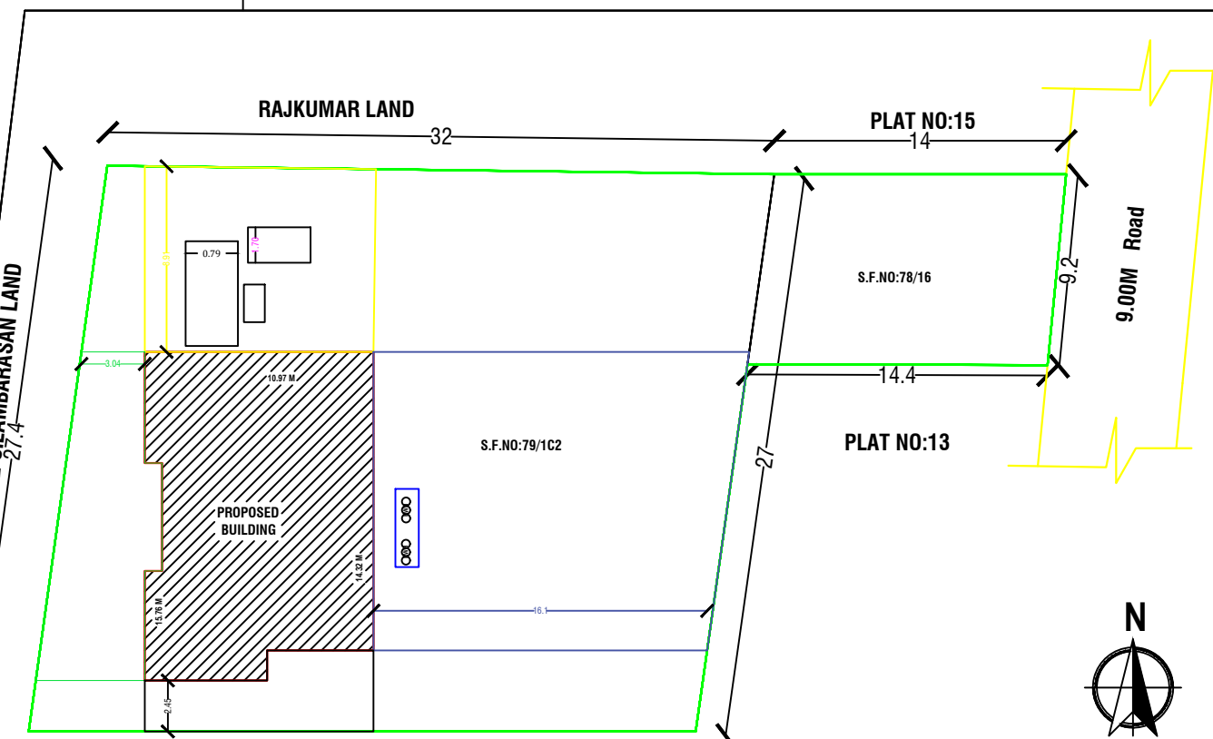
Site Plan
