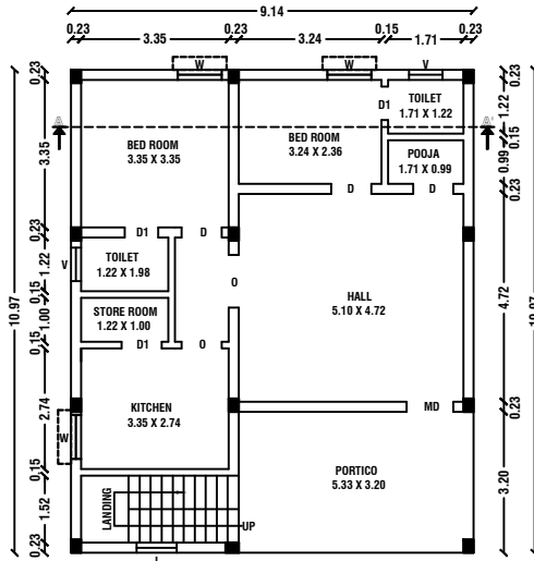
GROUND FLOOR PLAN (EXISTING BUILDING)
