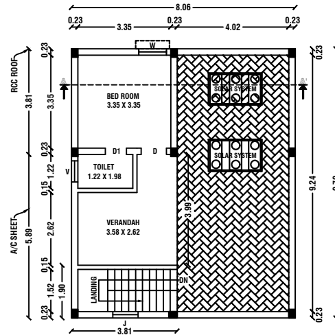
FIRST FLOOR PLAN (PROPOSED BUILDING)
