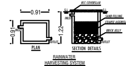
RAINWATER HARVESTING SYSTEM
