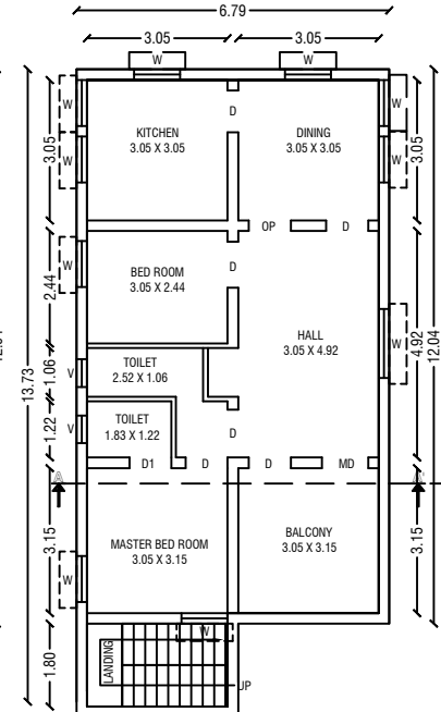
SECOND FLOOR PLAN (PROPOSED BUILDING)
