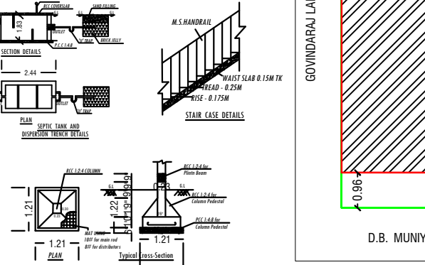
FOOTING DETAILS
