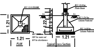
FOOTING DETAILS
