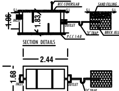
SEPTIC TANK AND DISPERSION TRENCH DETAILS
