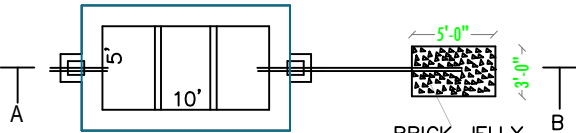
SEPTIC TANK & DISPERSION TRENCH DETAILS SCALE- 1:100
