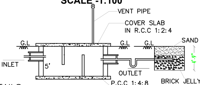
SECTION-AB
