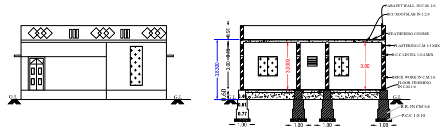
FRONT ELEVATION
