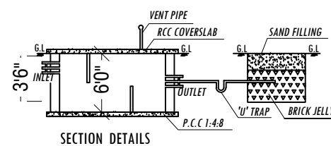
SECTION DETAILS
