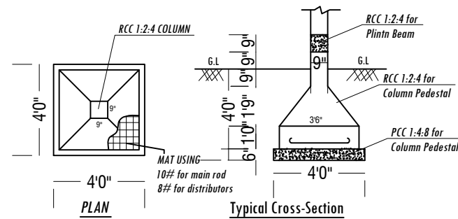
FOOTING DETAILS
