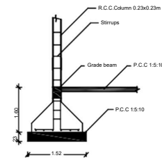
COLUMN DETAIL
