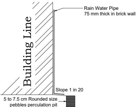
RAINWATER HARVESTING
