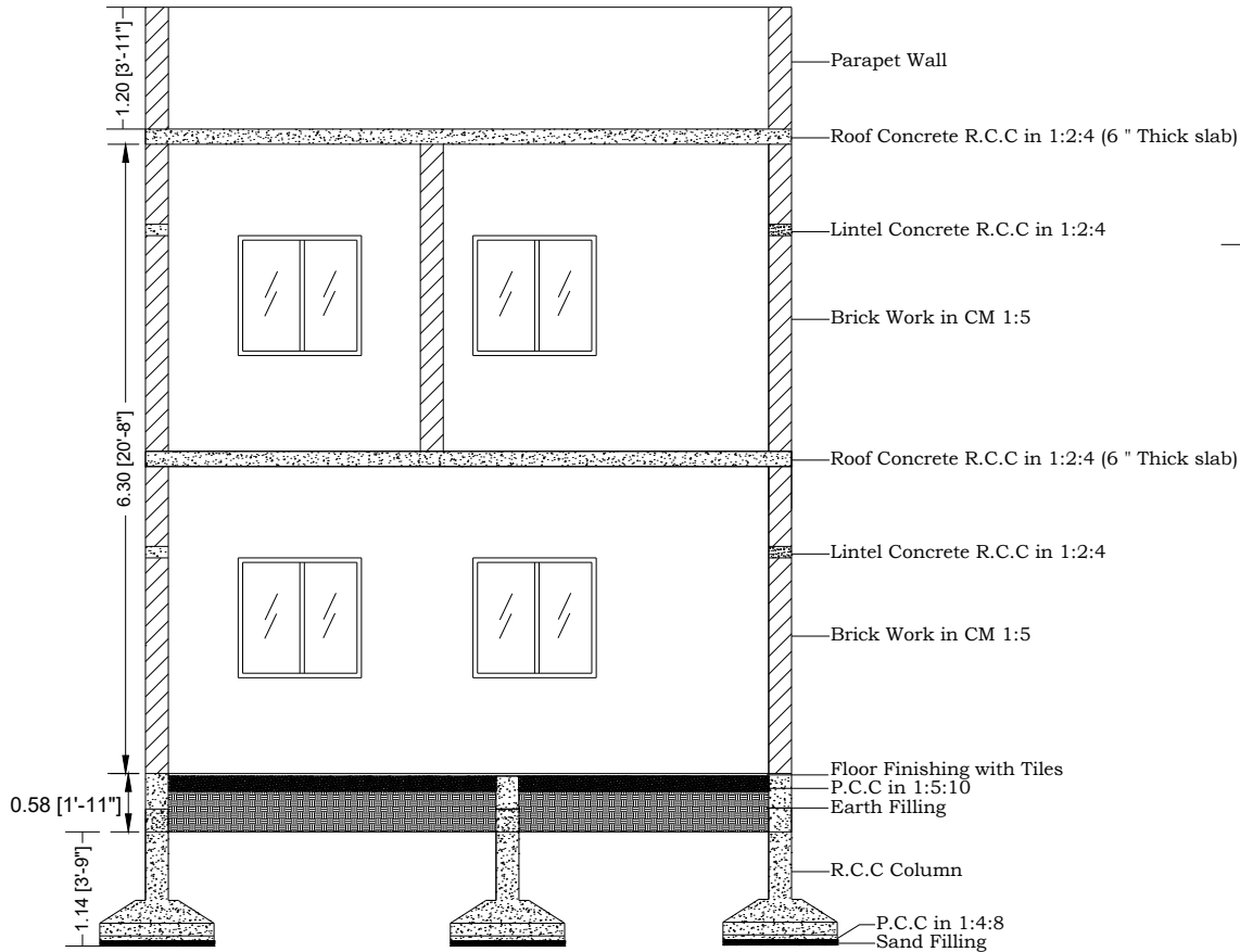
SECTION X-X
