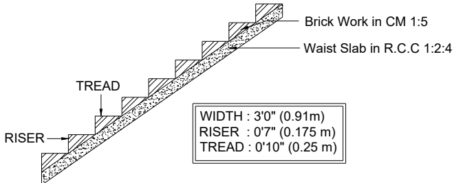
STAIRCASE DETAILS
