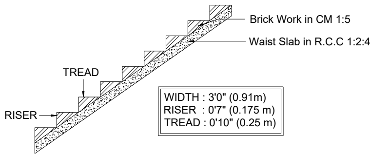
STAIRCASE DETAILS
