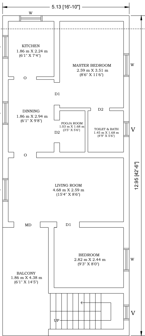
FIRST FLOOR
