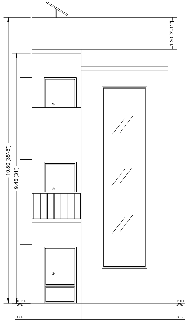
FRONT ELEVATION
