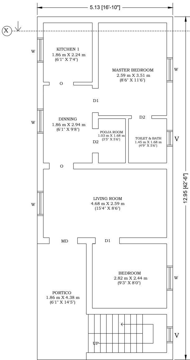
GROUND FLOOR
