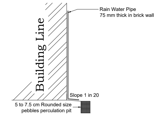
RAINWATER HARVESTING
