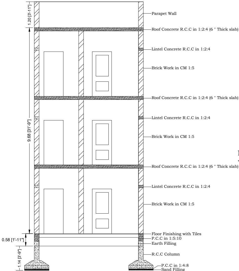
SECTION X-X
