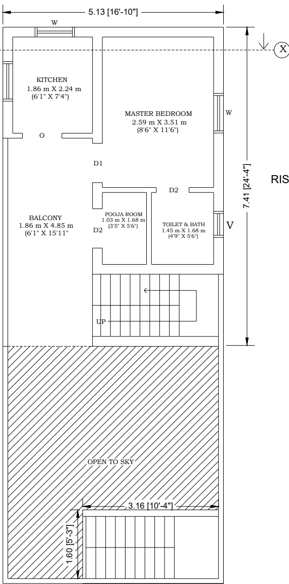
SECOND FLOOR
