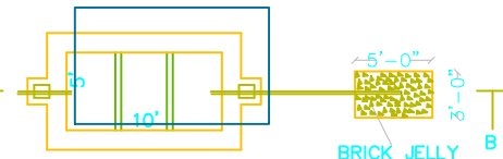
SEPTIC TANK & DISPERSION TRENCH DETAILS SCALE- 1:100
