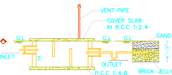
SECTION-AB
