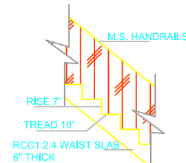
STAIRCASE DETAILS SCALE- 1:20
