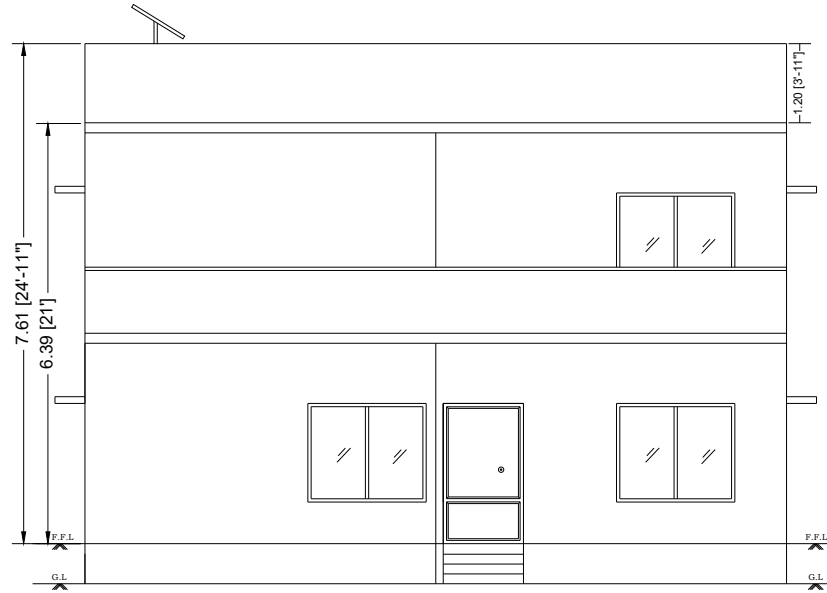
FRONT ELEVATION
