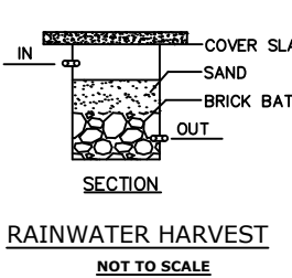
RAINWATER HARVEST NOT TO SCALE
