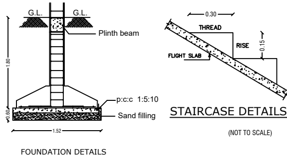
FOUNDATION DETAILS
