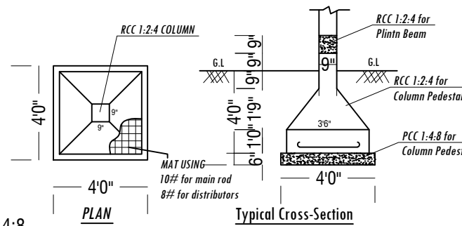
FOOTING DETAILS
