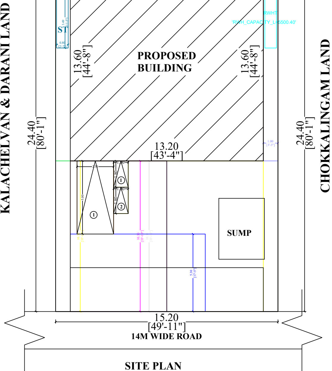
SITE PLAN
