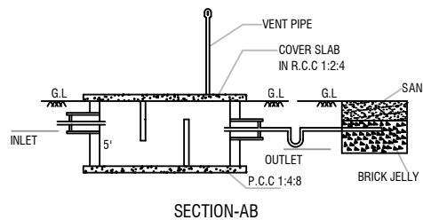
SECTION-AB
