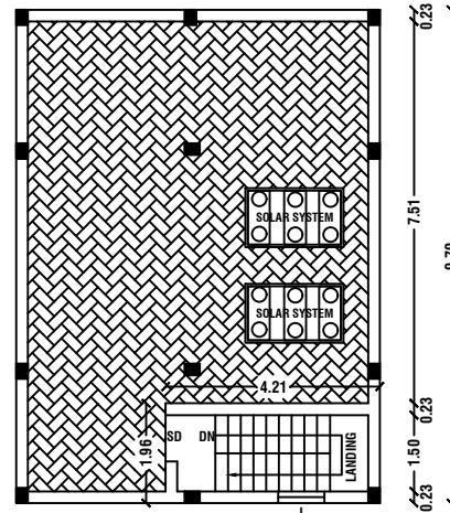
OPEN TERRACE FLOOR PLAN
