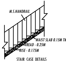
STAIR CASE DETAILS
