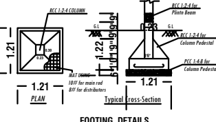
FOOTING DETAILS
