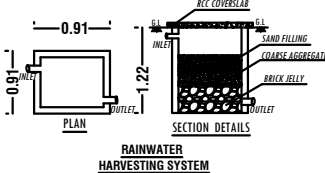
RAINWATER HARVESTING SYSTEM
