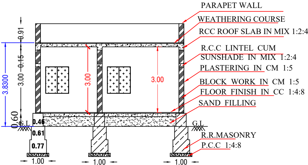
SECTION ON-"AB"
