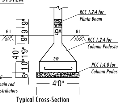
FOOTING DETAILS
