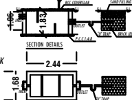
SECTION DETAILS
