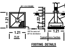
FOOTING DETAILS
