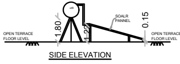
SIDE ELEVATION
