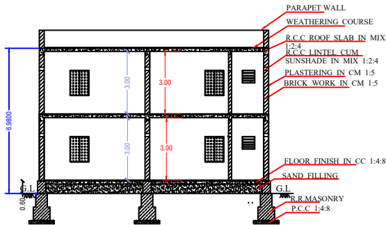
SECTION ON-"AB"
