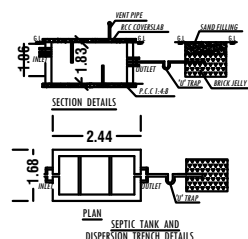
SEPTIC TANK AND DISPERSION TRENCH DETAILS
