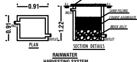
RAINWATER HARVESTING SYSTEM
