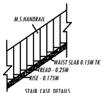
STAIR CASE DETAILS
