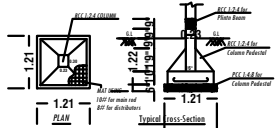
FOOTING DETAILS
