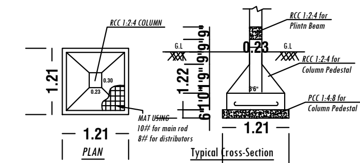
FOOTING DETAILS
