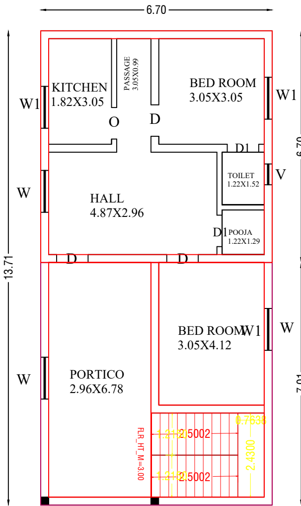
EXISTING AND PROPOSED GROUND FLOOR PLAN
