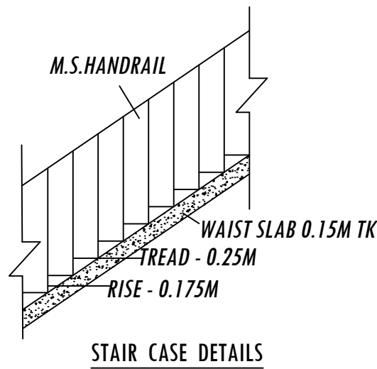
STAIR CASE DETAILS
