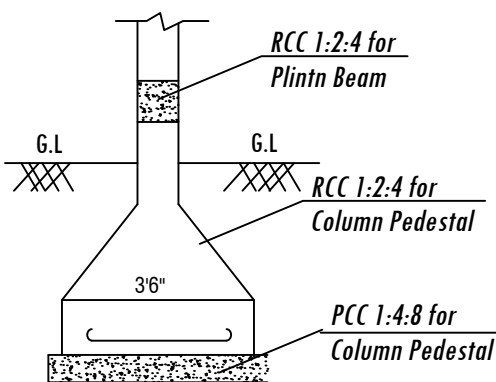
Typical Cross-Section FOOTING DETAILS
