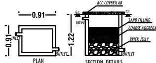
RAINWATER HARVESTING SYSTEM
