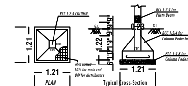
FOOTING DETAILS
