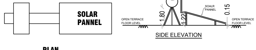
SOLAR WATER HEATER SCALE- 1:50
