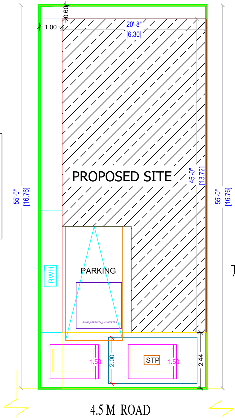
SITE PLAN
