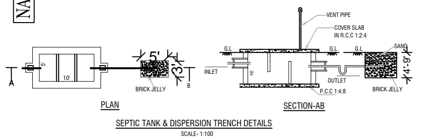
SEPTIC TANK & DISPERSION TRENCH DETAILS SCALE- 1:100
