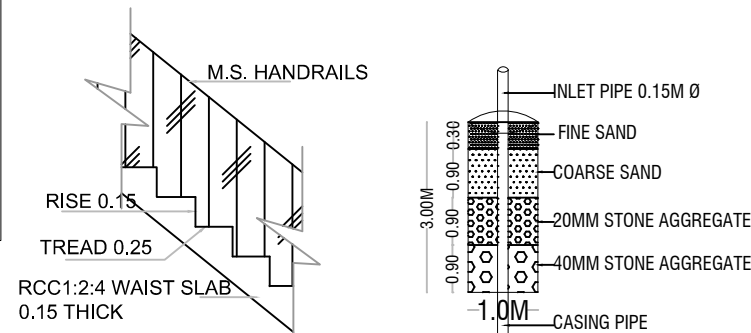
STAIRCASE DETAILS SCALE- 1:20
