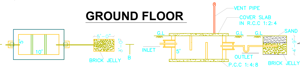
SEPTIC TANK & DISPERSION TRENCH DETAILS SCALE- 1:100
