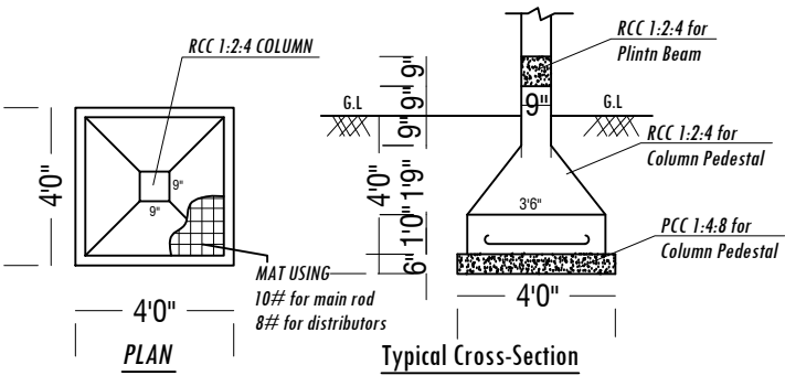
FOOTING DETAILS
