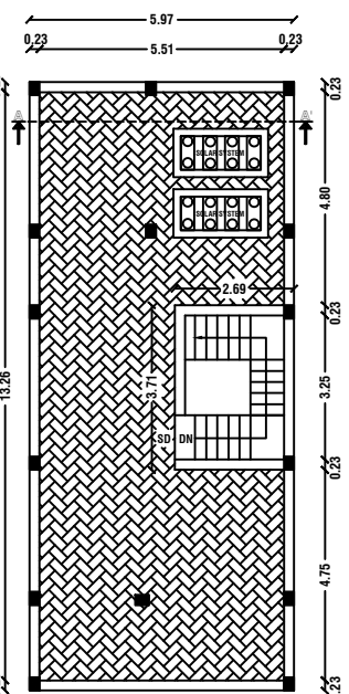
OPEN TERRACE FLOOR PLAN
