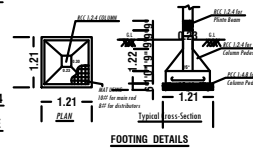
FOOTING DETAILS
