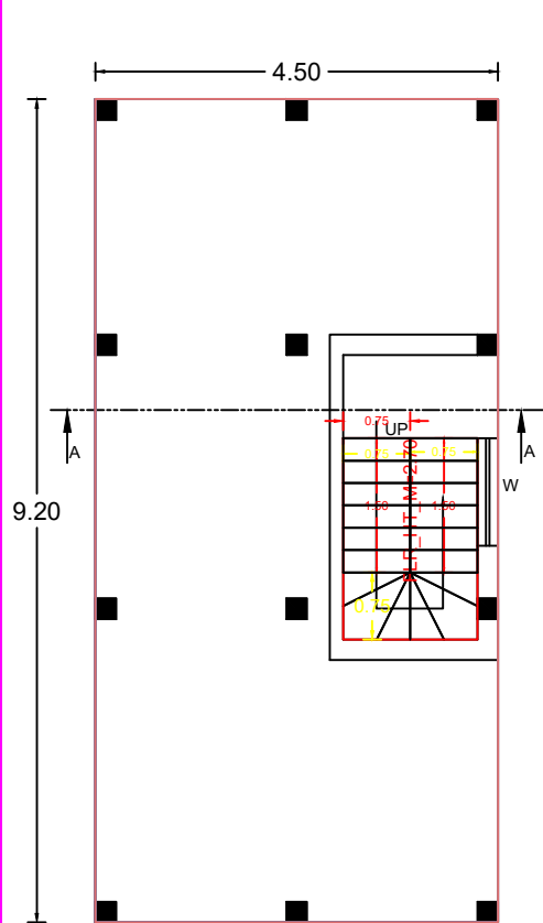
STILT FLOOR PLAN
