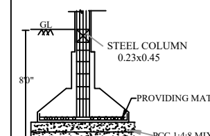
COLUMN FOOTING SCALE- 1:100
