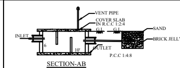
SEPTIC TANK & DISPERSION TRENCH DETAILS SCALE- 1:100
