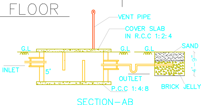
SECTION-AB
