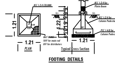
FOOTING DETAILS
