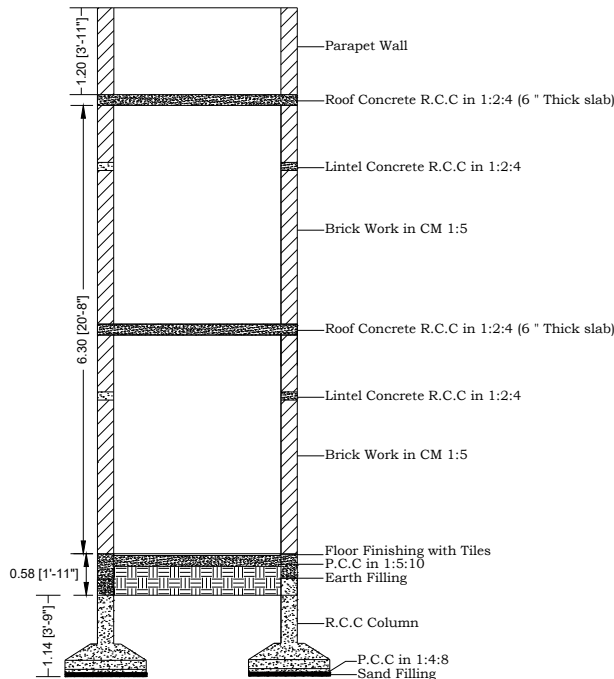
SECTION X-X
