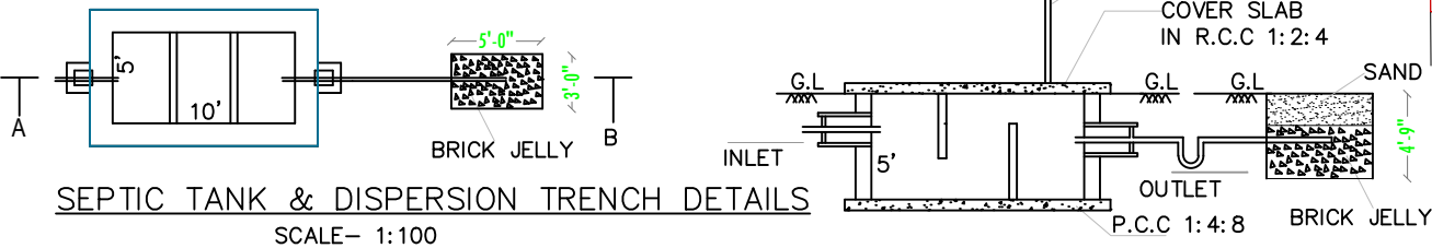
SECTION-AB
