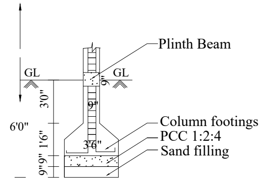
FOUNDATION DETAILS SCALE 1:50
