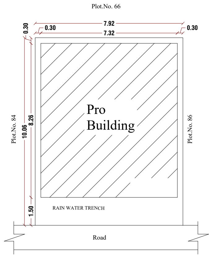
Sit Plan SCALE 1:100
