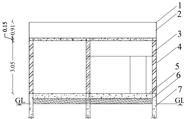
SECTION ON 'MS'
