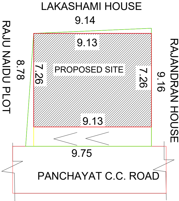
SITE PLAN
