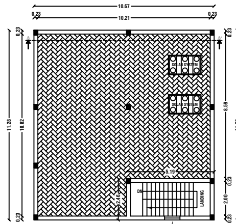
OPEN TERRACE FLOOR PLAN
