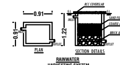
RAINWATER HARVESTING SYSTEM
