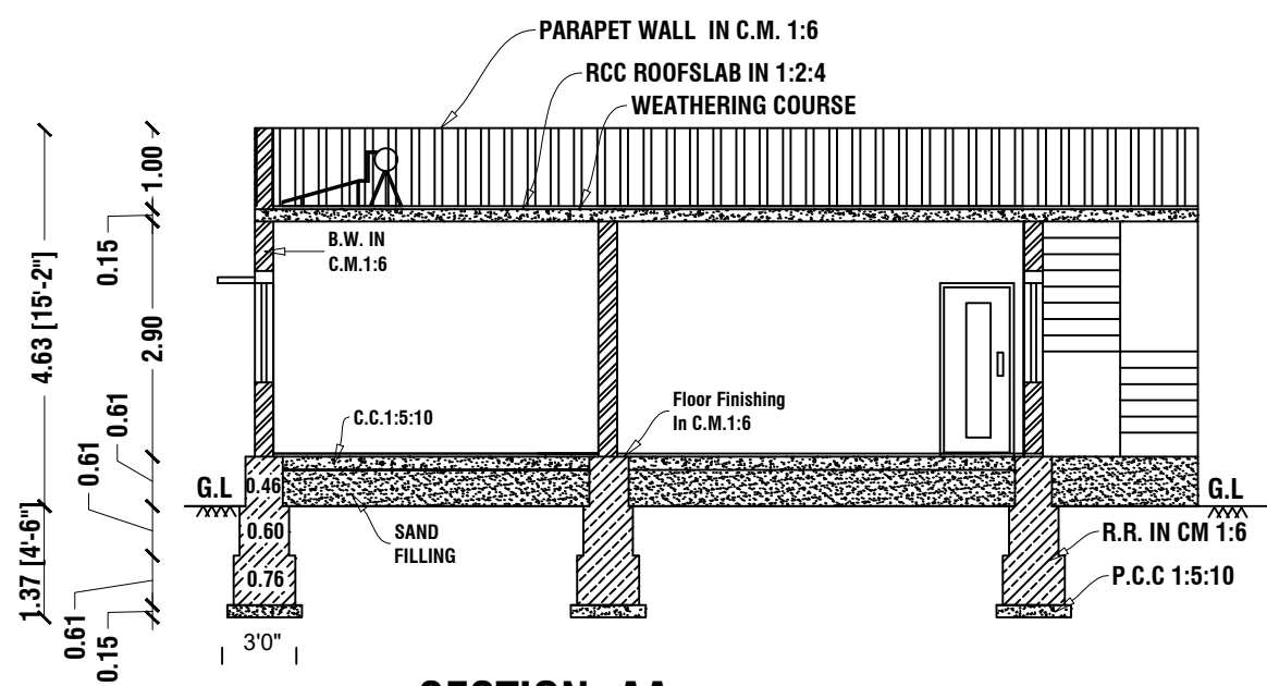
SECTION -AA
