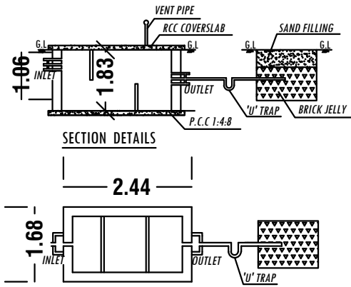
SEPTIC TANK AND DISPERSION TRENCH DETAILS
