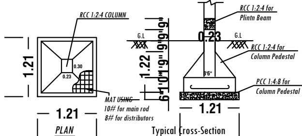
FOOTING DETAILS
