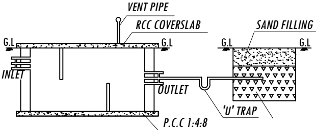
SECTION DETAILS
