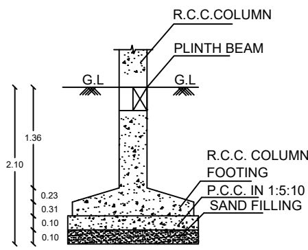
FOUNDATION DETAIL (DETAILS C)
