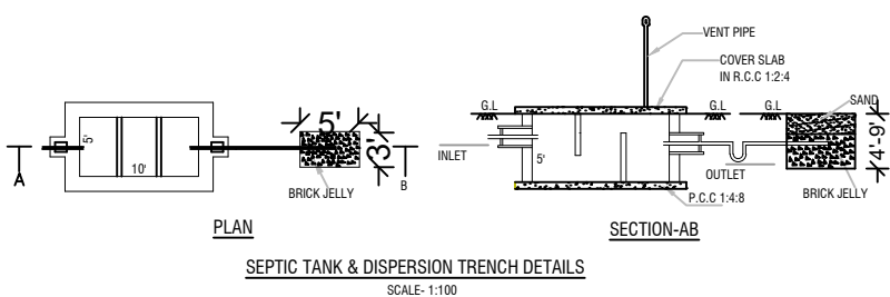
SEPTIC TANK & DISPERSION TRENCH DETAILS SCALE- 1:100
