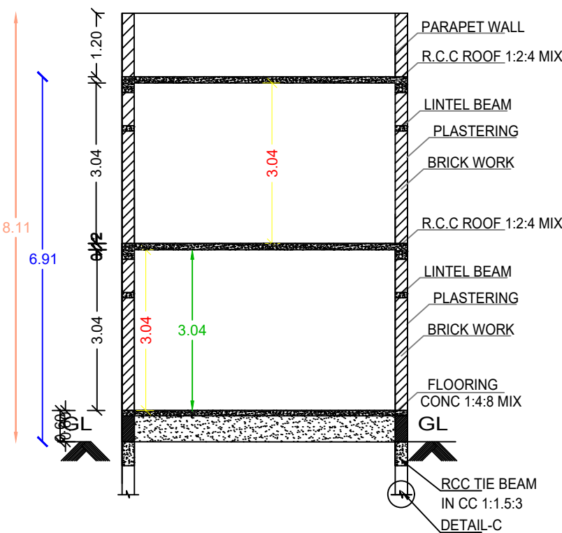
SECTION : "B-B"
