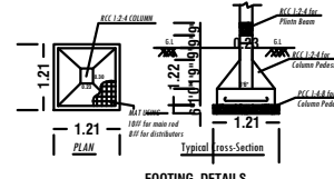
FOOTING DETAILS
