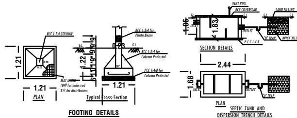
FOOTING DETAILS
